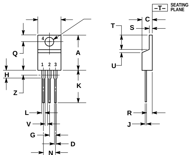
CASE 221A-09 (TO-220AB) ISSUE Z
